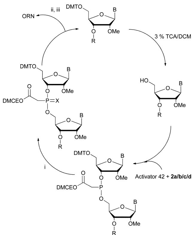
Scheme 2 Synthesis of PACE- and thioPACE-modified 2'- O -methyl-ORNs. (i) For X = O, 0.02 M I 2 /THF/pyridine/H 2 O; for X = S, 0.2 M phenylacetyl disulfide, acetonitrile/ N -methylimidazole 9:1. (ii) 1.5% DBU/acetonitrile, 1 h. (iii) 40% aqueous MeNH 2 , 55 °C, 15 min. B: a = A Bz , b = C Ac , c = G ibu , d = U. CPG = controlled-pore glass, DMCE = 1,1-dimethyl-2-cyanoethyl, DMT = 4,4'-dimethoxytrityl, TCA = trichloroacetic acid.
