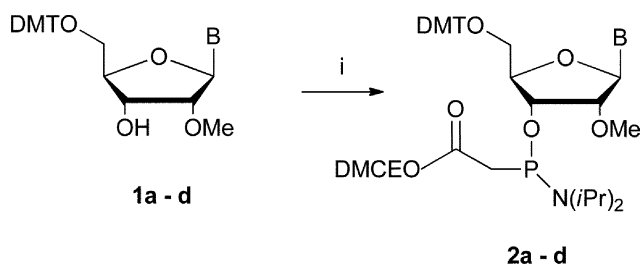
Scheme 1 Synthesis of 2'- O -methyl-3'- O -(diisopropylamino)phosphino acetic acid-1-dimethylcyanoethyl ester-5'- O -(4,4-dimethoxytrityl) ribonucleosides. (i) Acetic acid [bis( N,N -diisopropylamino)phosphino]-1,1-dimethyl-2-cyanoethyl ester, 4,5-dicyanoimidazole, dichloromethane. 2a 84% yield; 2b 79% yield; 2c 76% yield; 2d 95% yield. B: a = A Bz , b = C Ac , c = G Bu , d = U. DMCE = 1,1-dimethyl-2-cyanoethyl, DMT = 4,4'-dimethoxytrityl.
