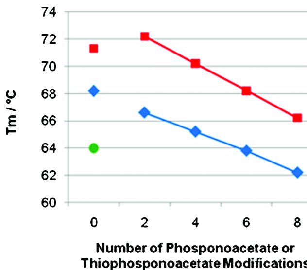
Fig. 2 Melting temperature ( T m ) of phosphonoacetate- and thiophosphonoacetate-modified oligoribonucleotides with complementary RNA. Melting temperatures were measured at 1 μM duplex in buffer which contained 0.1 M NaCl and 10 mM Na 2 HPO 4 . ● Unmodified RNA:RNA control; ■ RNA:phosphonoacetate ORNs 3–7; ◆ RNA:thiophosphonoacetate ORNs 8–12.
