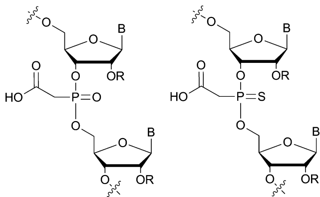
Fig. 1 General structure of phosphonoacetate (left) and thiophosphonoacetate (right) as oligodeoxynucleotide modifications; B = uridine (U), adenine (A), guanine (G) and cytosine (C).
