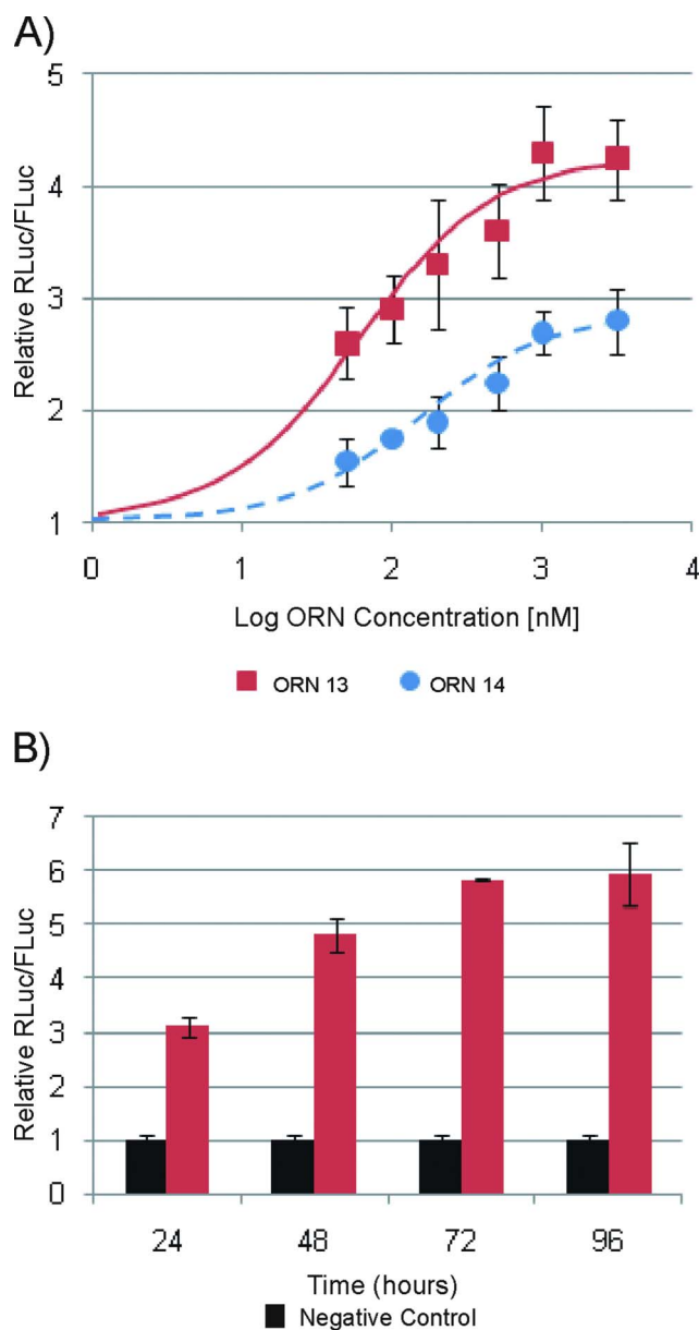
Fig. 8 Dose-response of miR-122 inhibition in Huh7 cells by ORNs 13 and 14 (top) and time dependence of miR-122 inhibition by 0.5 \mu M ORN 13 (bottom) as measured by a miR-122 sensor luciferase assay. Experiments were performed without lipid transfection. For dose–response, Huh7 cells expressing endogenous miR-122 were treated with ORNs at 0, 50, 100, 200, 500, 1000 and 3000 nM.
