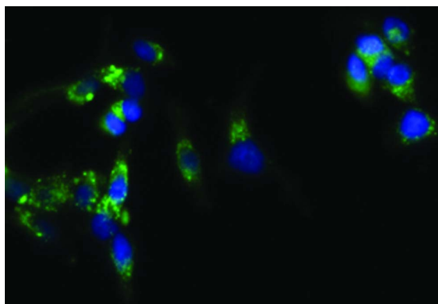
Fig. 7 Fluorescence microscopy image of HeLa cells incubated with fluorescently-labelled ORN 11 at 1 \mu\text{M} in the absence of a lipid transfecting agent. DAPI was used to stain the nuclei.
