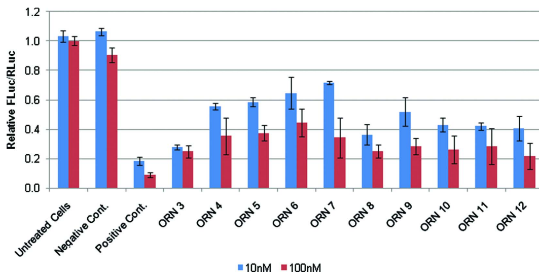
Fig. 3 siRNA activity of phosphonoacetate- and thiophosphonoacetate-modified ORNs as duplexes with siRNA in HeLa cells with lipid transfection as measured by down-regulation of firefly versus Renilla luciferase in a DualGlo luciferase assay. Positive control was AntiLuc siRNA1 (Dharmacon, Lafayette, CO), negative control was Silencer Negative Control 1 (Ambion, Foster City, CA). The concentrations indicated for untreated cells denote that the untreated cell experiments were run on the same plate as the cells that were treated with ORNs at the corresponding concentration.
